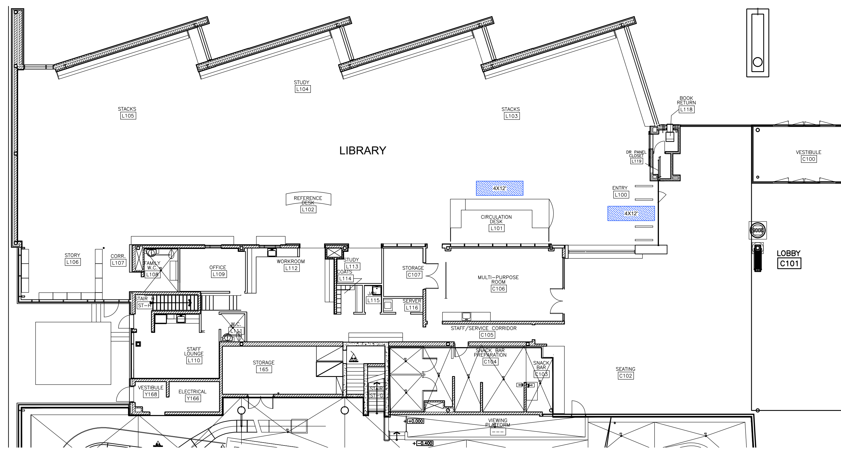
PARTIAL GROUND FLOOR PLAN N.T.S.
