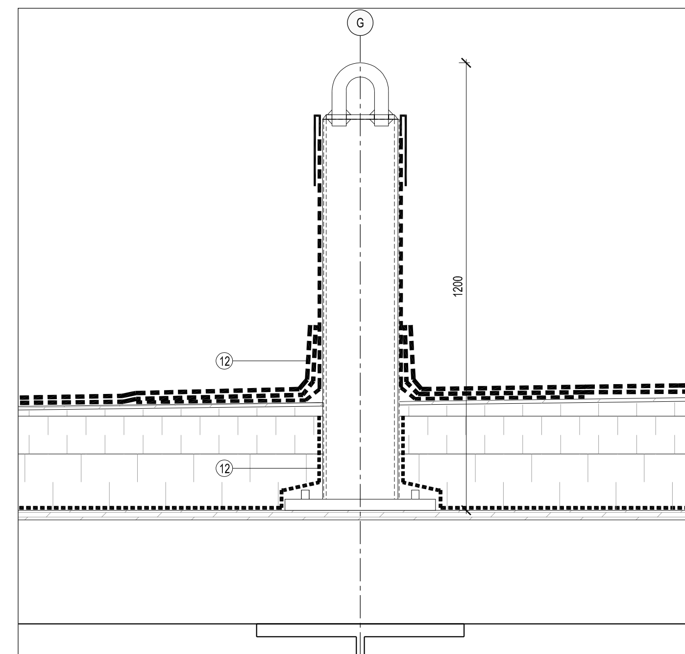
4 STEEL ROOF ANCHOR DETAIL A604 1:15
