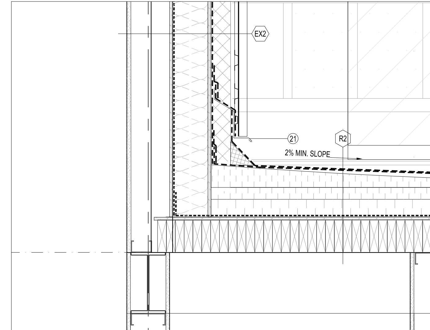
5 DETAIL SECTION THROUGH MARKET HALL BUILDING A604 1:10
