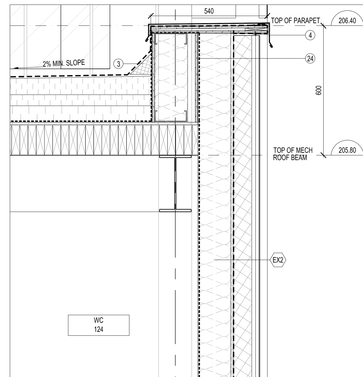
8 DETAIL SECTION THROUGH MARKET HALL BUILDING A604 1:10
