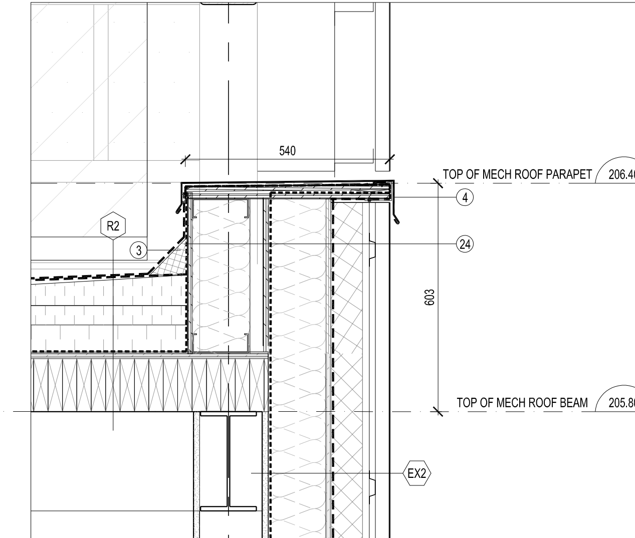
2 DETAIL SECTION THROUGH MARKET HALL BUILDING A604 1:10
