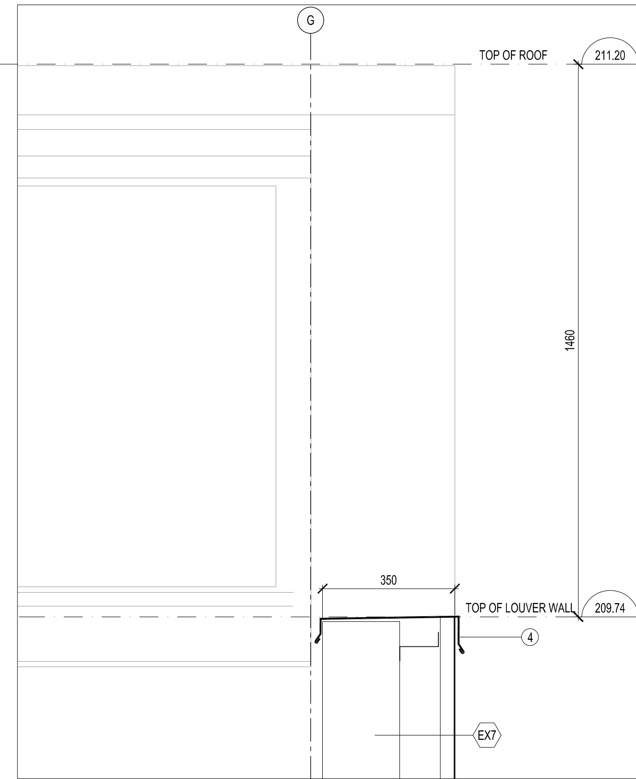
9 DETAIL SECTION THROUGH MARKET HALL BUILDING A604 1:10
