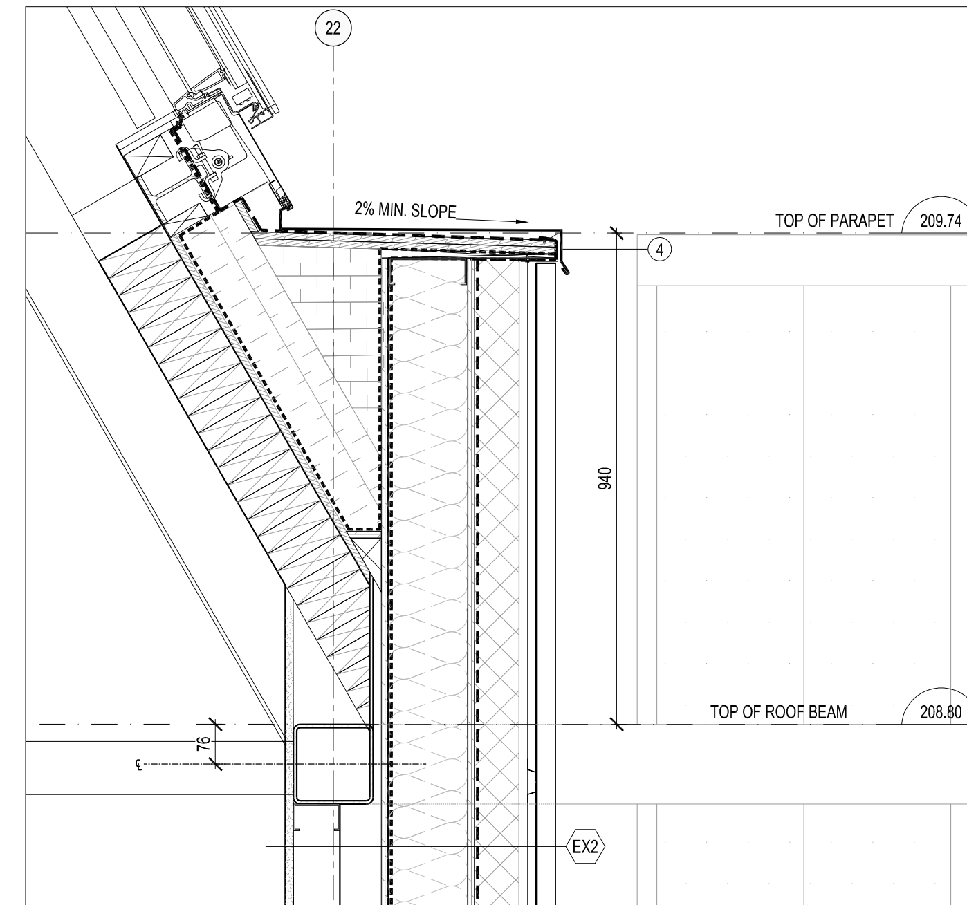
6 DETAIL SECTION THROUGH MARKET HALL BUILDING A604 1:10
