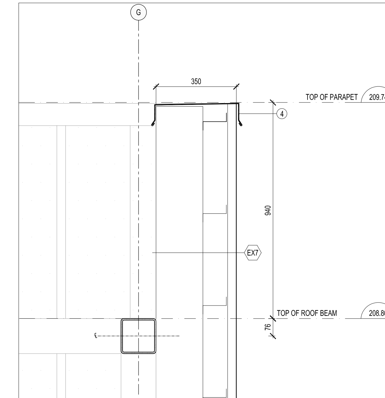
3 DETAIL SECTION THROUGH MARKET HALL BUILDING A604 1:10
