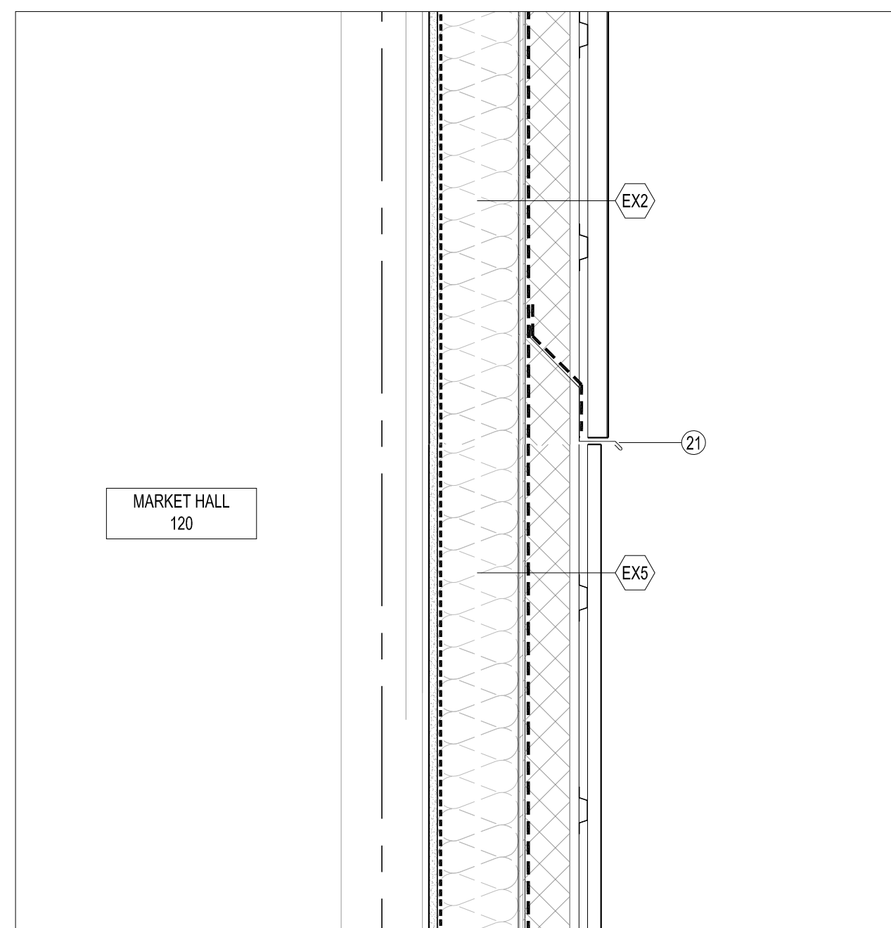
11 DETAIL SECTION THROUGH MARKET HALL BUILDING A604 1:10
