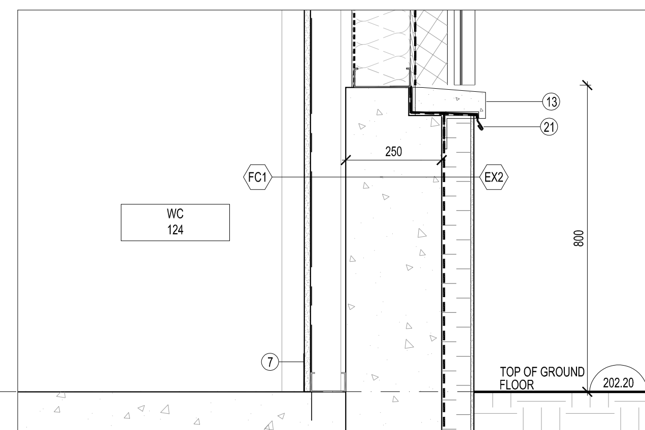
7 DETAIL SECTION THROUGH MARKET HALL BUILDING A604 1:10
