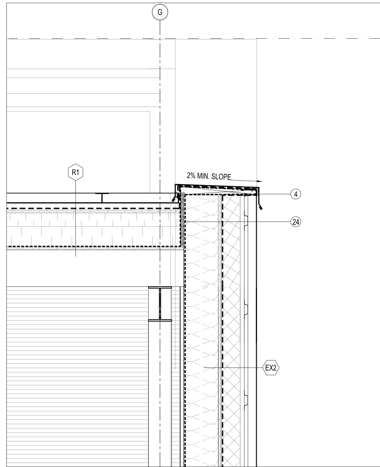
12 DETAIL SECTION THROUGH MARKET HALL BUILDING A604 1:10
