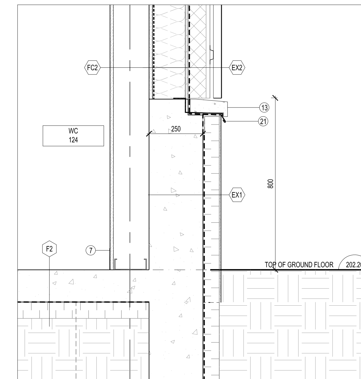
1 DETAIL SECTION THROUGH MARKET HALL BUILDING A604 1:10
