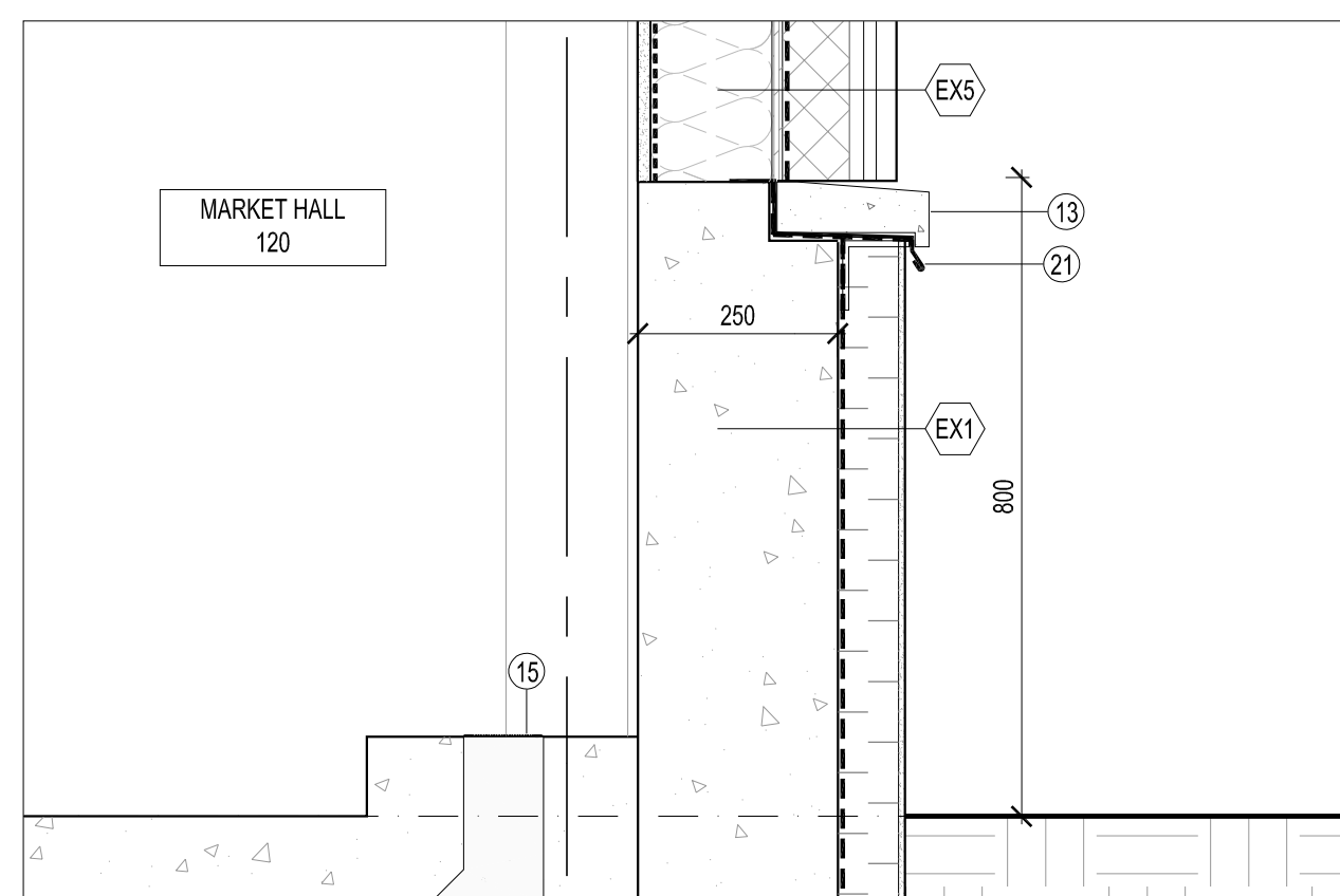
10 DETAIL SECTION THROUGH MARKET HALL BUILDING A604 1:10
