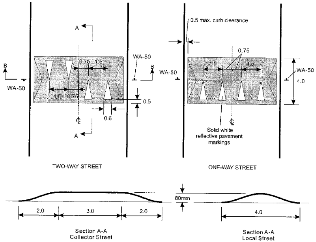
FIGURE 4.4 SPEED HUMP
