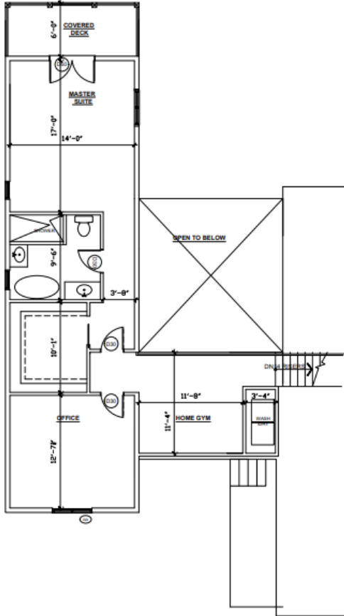
1 SECOND FLOOR PLAN 3/16" = 1'-0"
