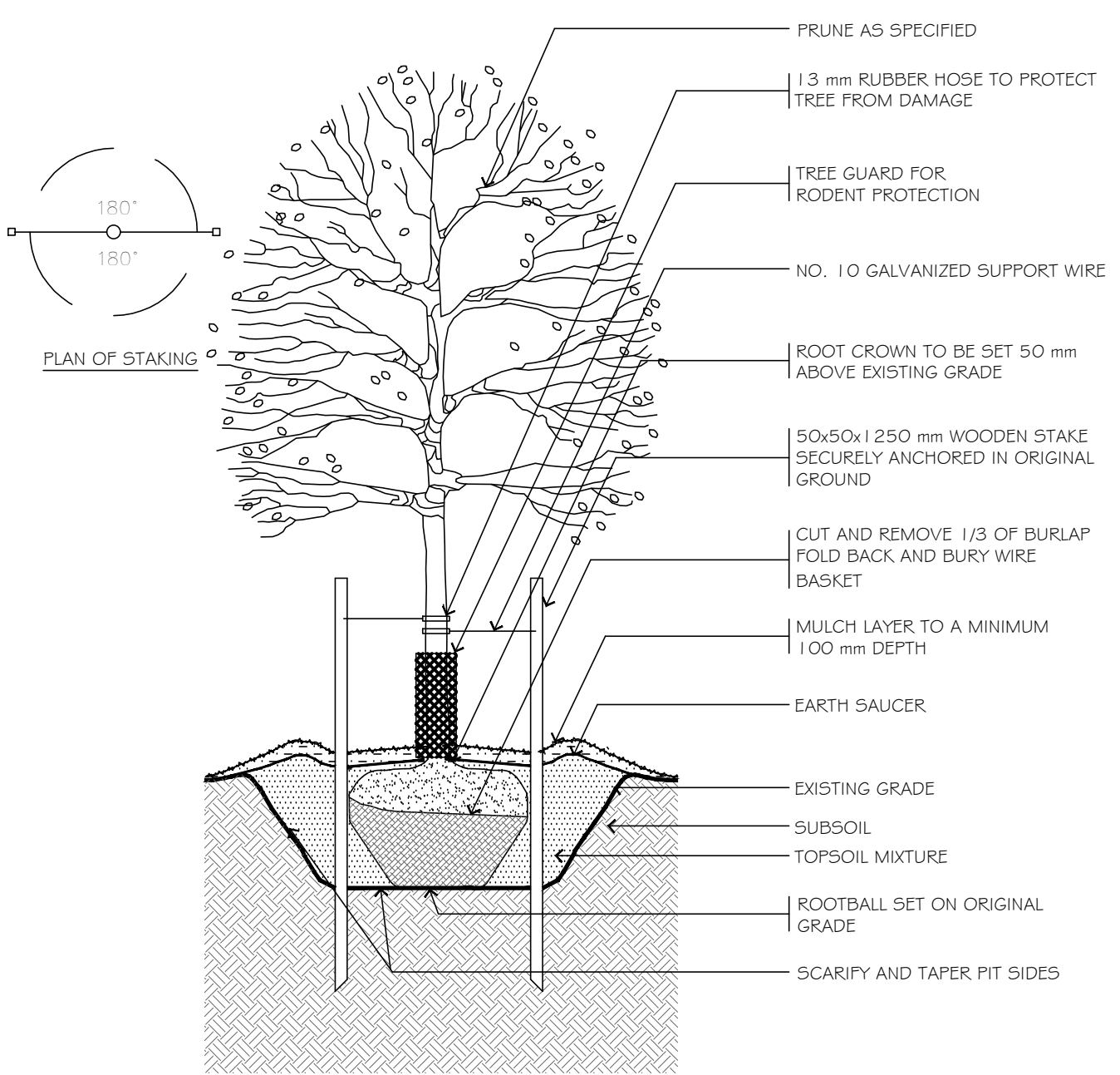
D2 TYPICAL DECIDUOUS TREE PLANTING DETAIL TREES OVER 45mm CALIPER SCALE: NONE
