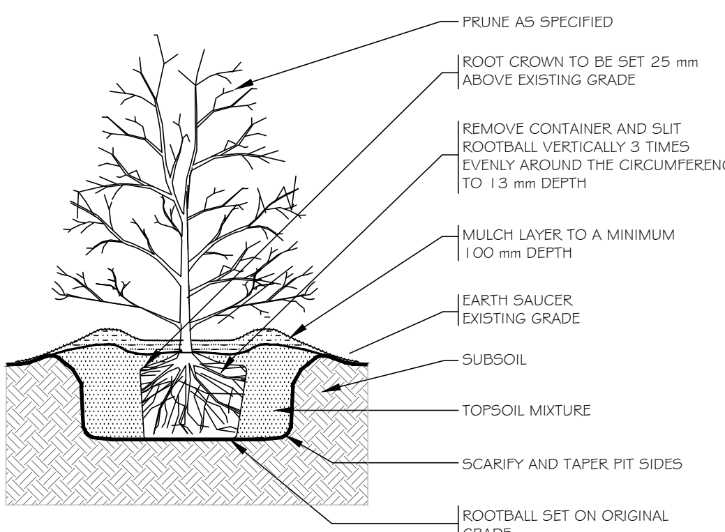
D1 TYPICAL SHRUB PLANTING DETAIL ALL SPECIES / SIZES SCALE: NONE
