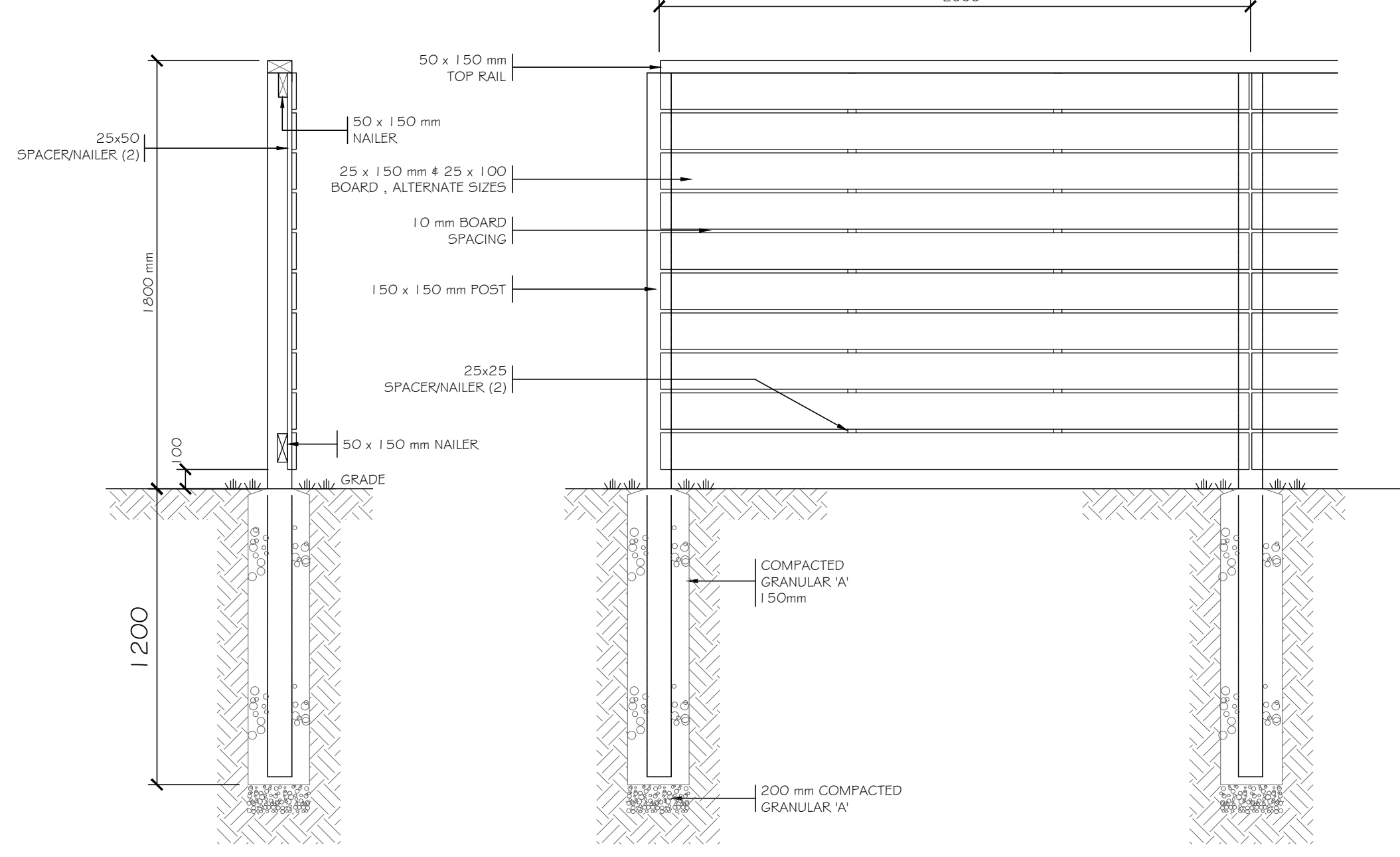
D3 TIMBER (CEDAR) PERIMETER FENCE DETAIL (TIMBER POSTS TO BE PRESSURE TREATED) SCALE: NONE
