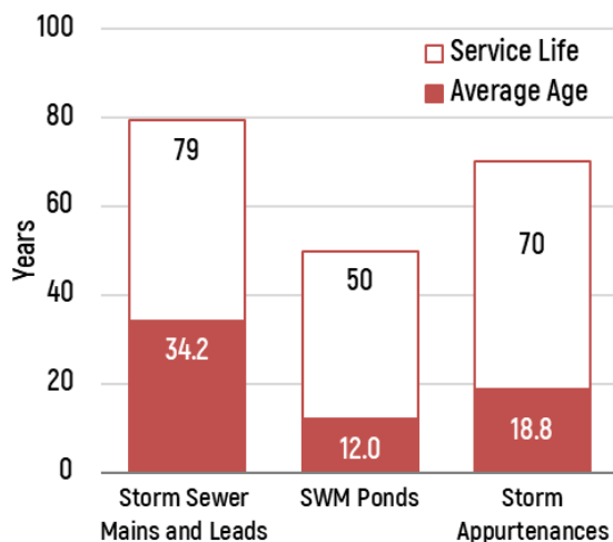
Figure 2-7 Average Age & Estimated Life of Stormwater Mgmt System
