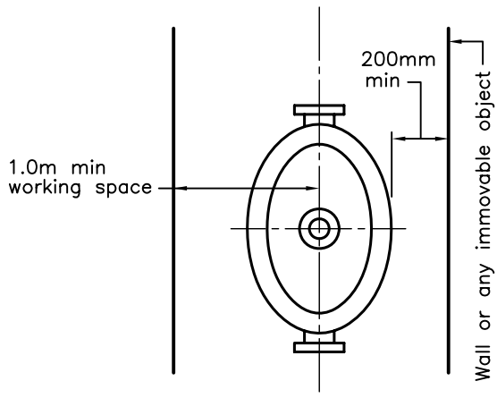
TOP VIEW OF METER
