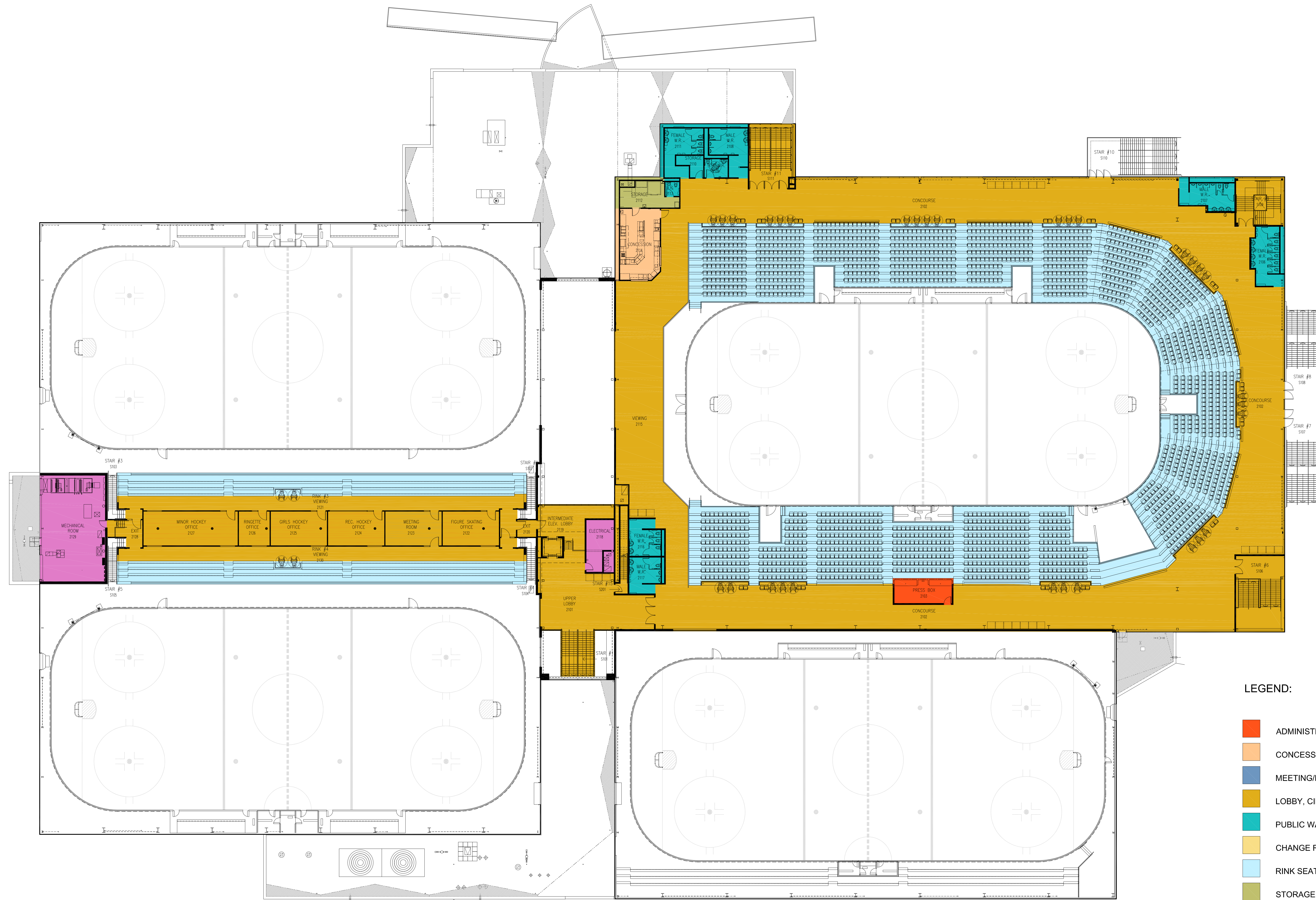
UPPER FLOOR PLAN
